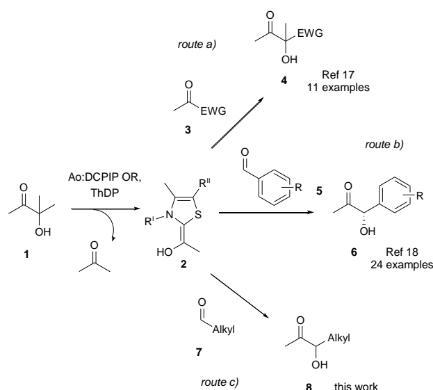
Scheme 2. Ao:DCPIP OR catalyzed benzoin-type condensation of methylacetoin ( 1 ) with activated ketones (route a), aromatic aldehydes (route b) and aliphatic aldehydes (route c). R^I = (4-amino-2-methylpyrimidin-5-yl)methyl, R^{II} = 2-diphosphate ethyl.
