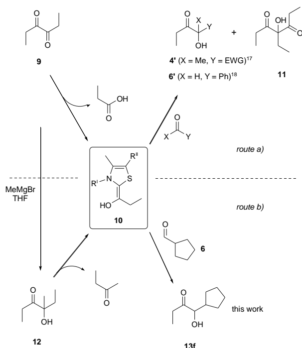
Scheme 3. Synthesis and exploitation of 4-hydroxy-4-methylhexan-3-one ( 12 ) as a propionyl anion donor alternative to hexane-3,4-dione ( 9 ). R^I = (4-amino-2-methylpyrimidin-5-yl)methyl, R^{II} = 2-diphosphate ethyl.
