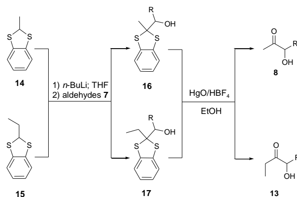
Scheme 4. Synthesis of racemic samples of products 8c,d,g,h,j and 13c,d,f,h,j .
