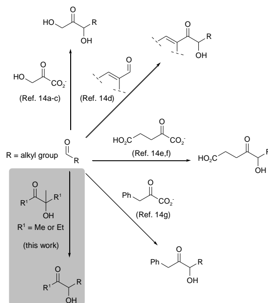
Scheme 1. Generic structures of the main aliphatic acyloins achievable via ThDP-dependent enzyme catalysis.
