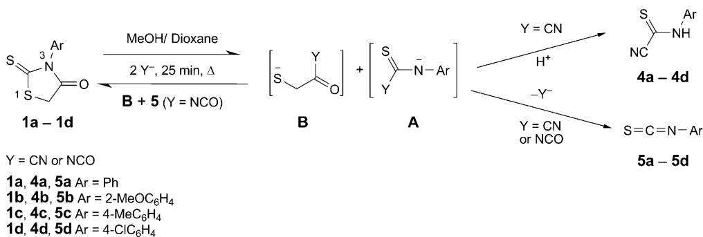
Scheme 1. Reactions of 1a–1d with KCN and KOCN
