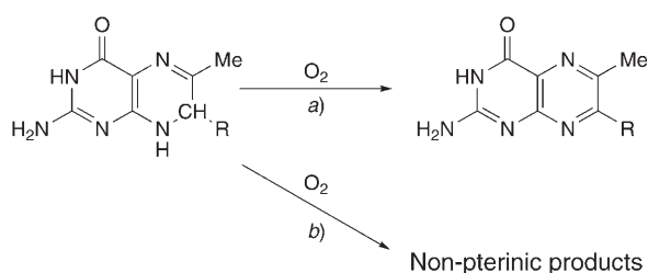
Scheme 2. Oxidation of 7,8-Dihydro-6-methylpterin ( \text{R} = \text{H} ) and 7,8-Dihydro-6,7-dimethylpterin ( \text{R} = \text{Me} ) by \text{O}_2 in Neutral Aqueous Solution
