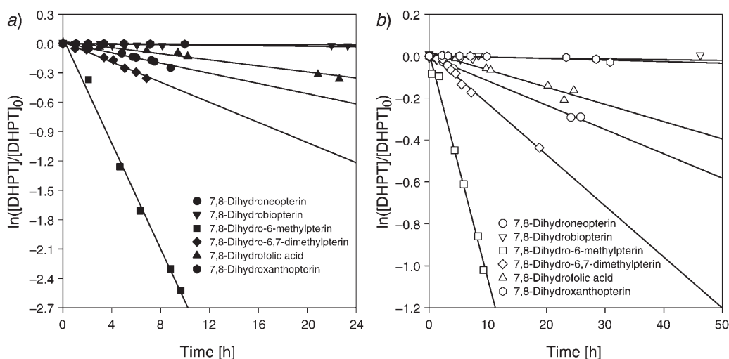
Fig. 8. First-order plots of the oxidation of the 7,8-dihydropterins derivatives (DHPT) in air-equilibrated aqueous solutions (Eqn. 2, Exper. Part). Concentrations of dihydropterins determined by HPLC analysis, pH 7.0 \pm 0.1 . a) T = 40^\circ . b) T = 25^\circ .
