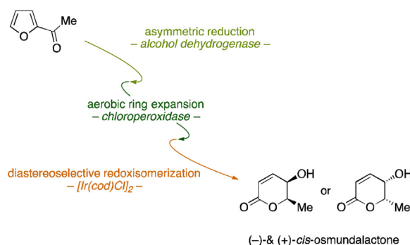
Scheme 1. Triple-catalytic strategy towards stereodefined osmundalactones.
