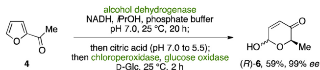
Scheme 3. Sequential reduction/rearrangement cascade with intermediate pH adjustment.
