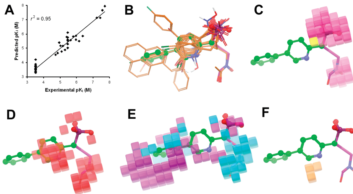
Figure 3. (A) Correlation between the experimental Ec DXR inhibitory activity and predicted activity by the phase QSAR model, showing r^2 = 0.95 . (B) Flexible alignment of compounds (only heavy atoms and polar hydrogens displayed for clarity), with compound 9 shown in a ball and stick model and 1 in a tube model. (C) Phase negative ionic fields, pink favorable, yellow disfavored. (D) Electron-withdrawing fields, red favorable. (E) Hydrophobic fields, cyan favorable, purple disfavored. (F) H-bond donor fields, orange disfavored.
