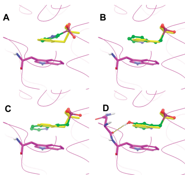
Figure 2. Lowest energy docking structures of compounds (A) 11, (B) 12, (C) 13, and (D) 30 in the EcDXR :8 structure, together with superimposed structure of 8 (in yellow).
