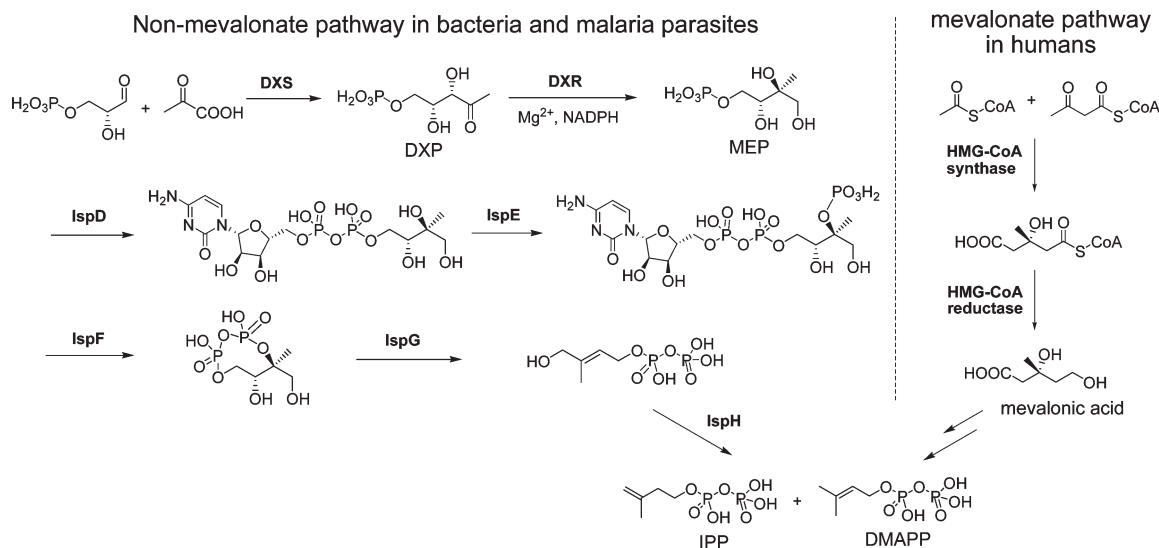
Figure 1. Non-mevalonate and mevalonate isoprene biosynthesis pathways.
