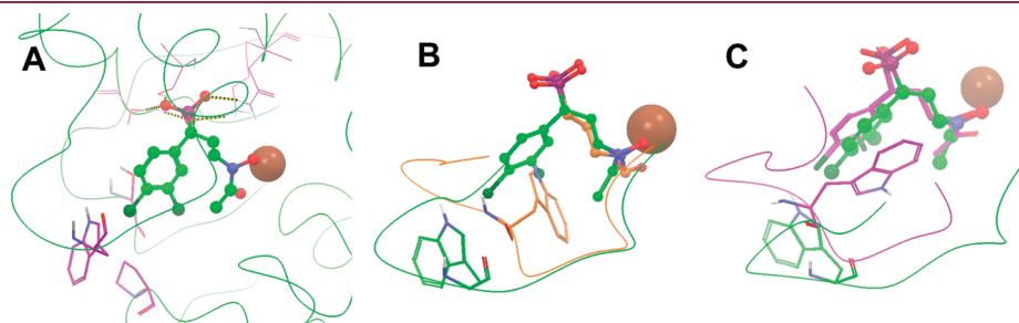
Figure 4. (A) Active site of the MtDXR : 4 structure. The protein backbone is shown as green curved lines, 4 as a ball and stick model, and \text{Mn}^{2+} as a brown sphere. (B) Crystal structure of MtDXR : 4 (in green) superimposed with the structure of MtDXR : 1 (in orange). For clarity, only the flexible loops containing residues 198–208 of the two structures are shown as curved lines. (C) Crystal structure of MtDXR : 4 (in green) superimposed with a modeled structure of EcDXR : 4 complex (in purple). Only the flexible loops (residues 198–208 for MtDXR and 205–215 for EcDXR ) of the two structures are shown as curved lines.
