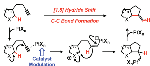
Scheme 1. Platinum-Catalyzed Coupling of Unactivated Alkynes and \text{sp}^3 C–H Bonds via the Through-Space Hydride Transfer
