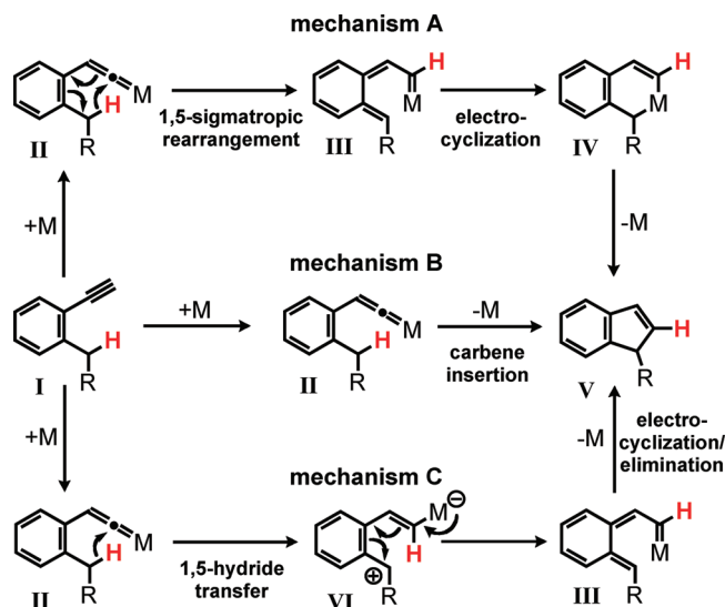
Scheme 2. Cyclization of 2-Alkyl-1-ethynylbenzenes and Proposed Mechanistic Rationales
