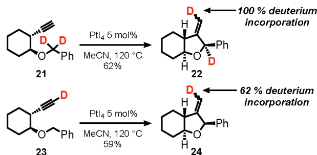
Scheme 3. HT-Cyclization of Deuterium Labeled Compounds 21 and 23
