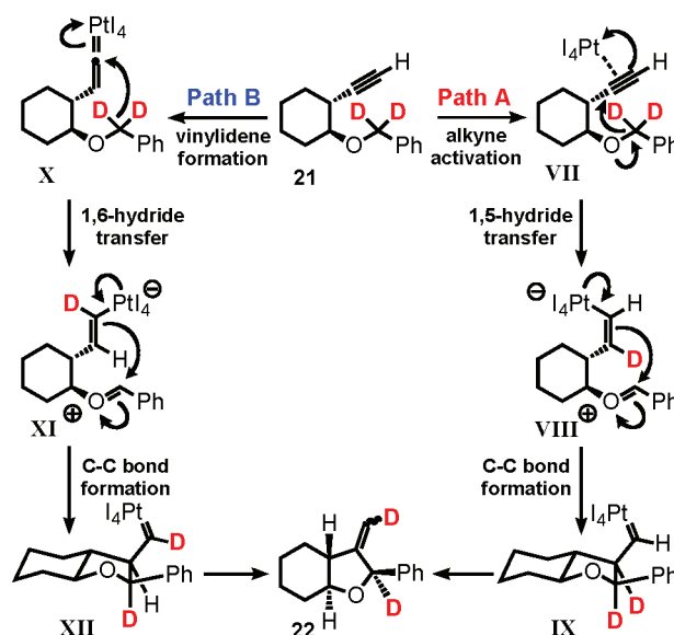
Scheme 4. Proposed Mechanisms for the Platinum-Catalyzed HT-Cyclization
