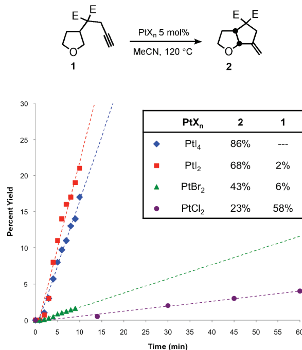
Figure 1. Effect of halide ligand on the catalyst activity. Initial rates of product 2 formation are shown in the plot. The inset lists the yields of product 2 and remaining starting material 1 . Reactions performed at 0.05 M in dry MeCN. Yields were determined by GC, employing tetrachlorobenzene as an internal standard. E = CO 2 Me.
