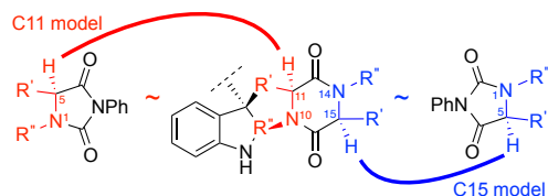
Figure 5. Structural correlation used to calculate parameters for hydantoin and the corresponding diketopiperazines.
