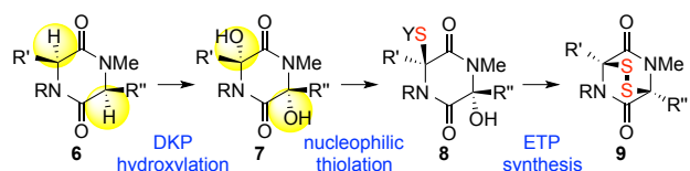
Scheme 1. Key steps in the conversion of diketopiperazines (DKPs) to the corresponding epithiodiketopiperazines (ETPs).
