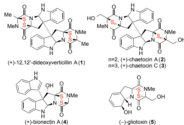
Figure 1. Representative epipolythiodiketopiperazine natural products.
