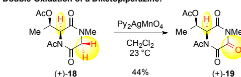
Scheme 2. Representative application of our permanganate-mediated diketopiperazine oxidation chemistry.
