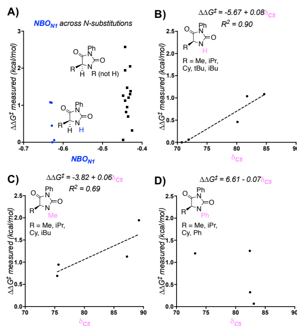
Figure 4. The NBO charge of N 1 describes the N1-H subset (A) and the 13 C NMR shift describes variation in the C5 substituent (B,C,D).
