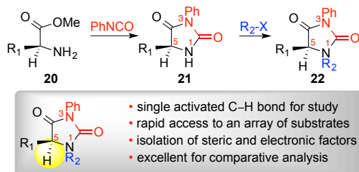
Scheme 3. General preparation of hydantoin.
