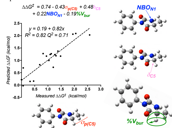
Figure 2. Model comparing predicted \Delta\Delta G^\ddagger to measured \Delta\Delta G^\ddagger for the hydantoin library utilizing the Taft parameter \sigma_p , a nitrogen NBO charge, a 13 C NMR shift, and percent buried volume of the abstracted hydrogen.
