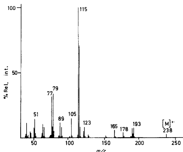
Figure 1. 70 eV mass spectrum of 1-(3-phenyl-2-propynyl)-1,4-dihydrobenzoic acid (3).
