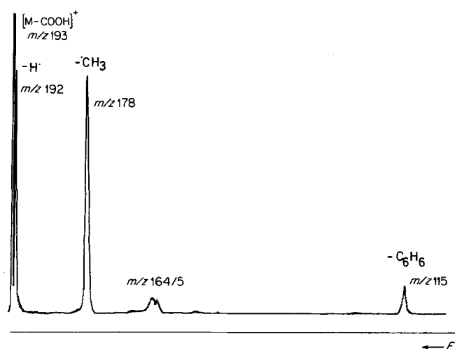
Figure 2. MIKE spectrum of (3-phenyl-2-propynyl)-1-benzenium ions b (from 3).
