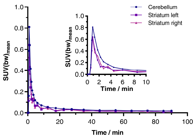
Figure 4. TAC for [ ^{68}\text{Ga} ]Ga-HBED-hexadiyne-tropane 13 for right and left striatum.
