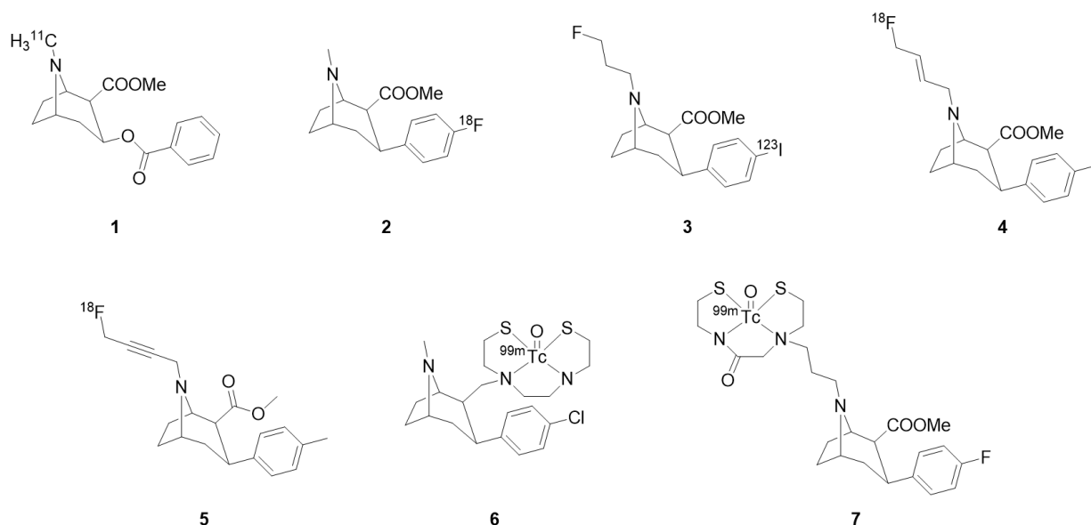
Figure 1. Representative tropene derivatives established for PET imaging of the hDAT.
