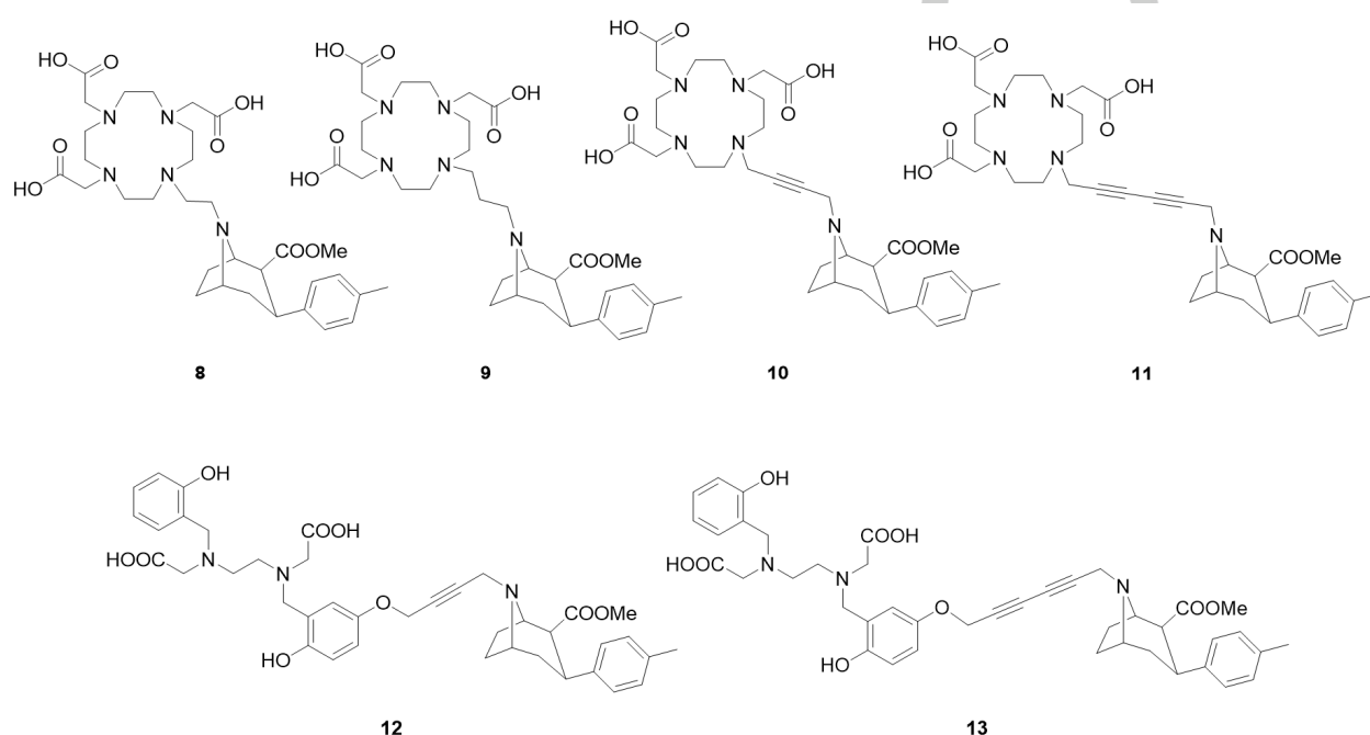
Figure 2. DO3A- and HBED-coupled tropane derivatives for 68 Ga-labelling.
