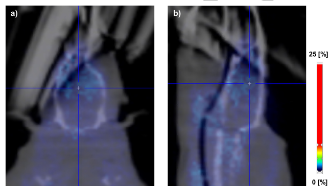
Figure 3. \mu\text{PET}/\text{CT} image of [ ^{68}\text{Ga} ]Ga-HBED-hexadiyne-tropane 13 in a 6-OHDA-rat 60 min p.i.; a) coronal; b) sagittal.
