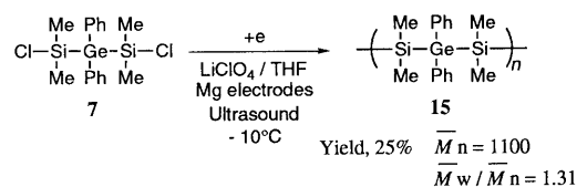
Scheme 9.
