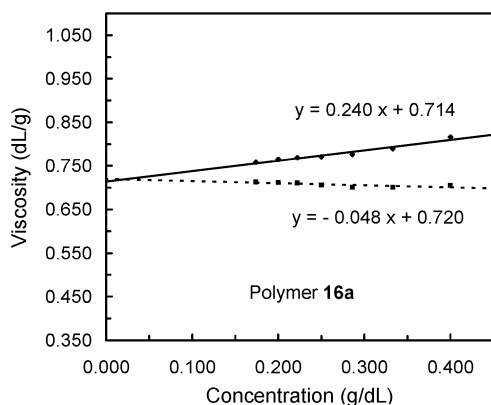
FIGURE 9. Plots of inherent viscosity \eta_{\text{inh}} and reduced specific viscosity \eta_{\text{sp}}/c vs concentration of poly(bibenzimidazole) ( 16a ) at 30.00 °C in methanesulfonic acid. Solid line: \eta_{\text{red}} = \eta_{\text{sp}}/c . Dotted line: \eta_{\text{inh}} = (\ln \eta_r)/c .
