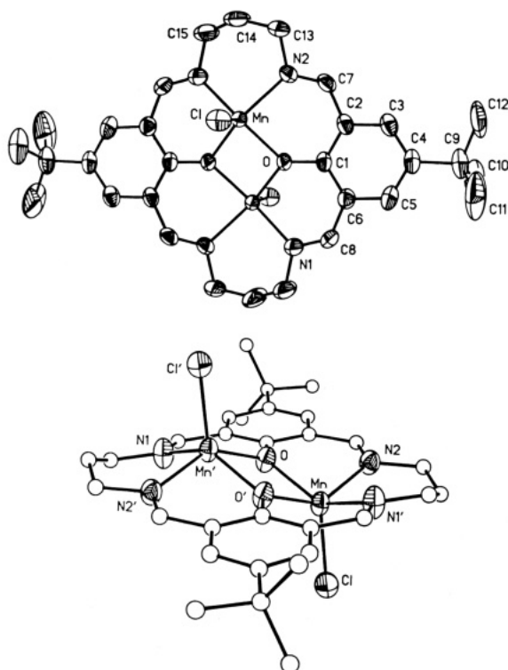
Figure 1. (Upper) ORTEP plot showing the planar structure of \text{LMn}_2\text{Cl}_2 (4). (Lower) View from the side of \text{LMn}_2\text{Cl}_2 (4) showing the displacement of the manganese atoms from the plane of the macrocyclic ligand.
