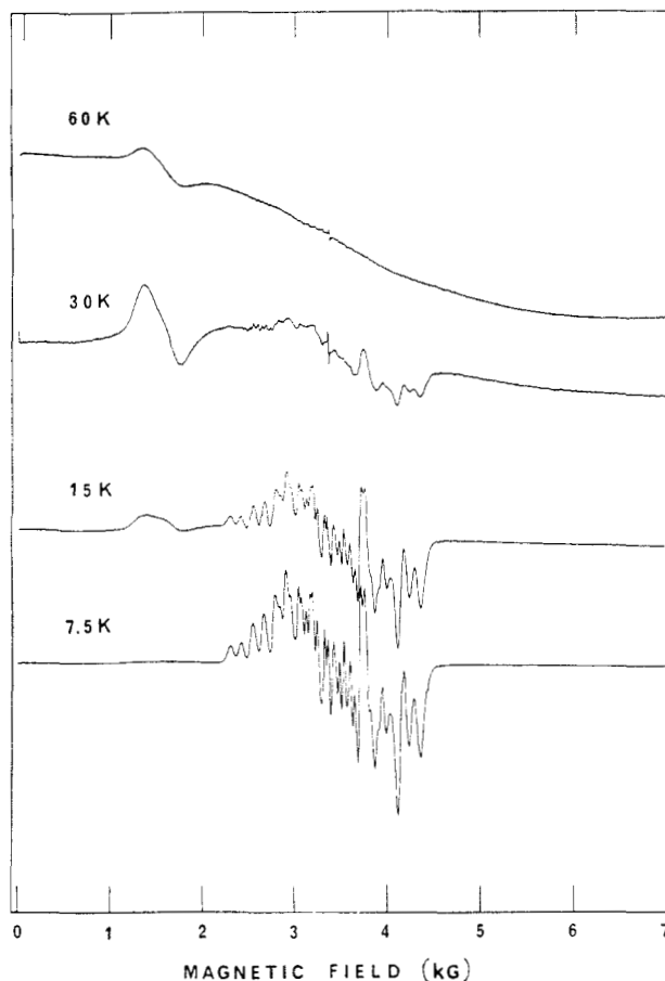
Figure 8. Variable-temperature X-band EPR spectrum of [Mn_2-(bpm)(\mu-OAc)_2](ClO_4)_2 \cdot H_2O (1) in acetone/toluene/ethanol glass.
