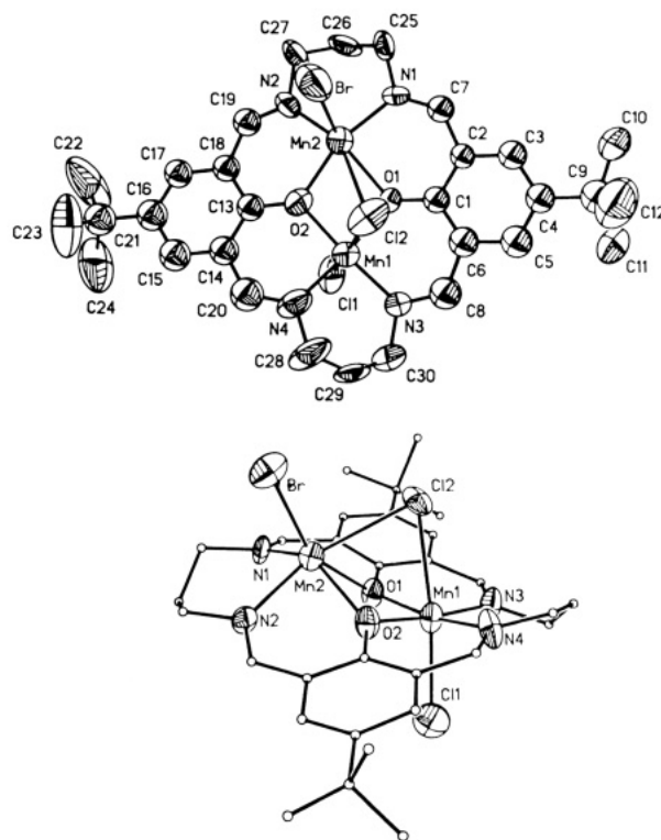
Figure 2. (Upper) ORTEP plot showing the planar structure of [\text{LMn}_2\text{Cl}_2\text{Br}]\cdot\text{H}_2\text{O} (2) and the distorted trigonal prismatic coordination geometry of \text{Mn}_2 . (Lower) View showing the disposition of the manganese atoms with respect to the plane of the macrocyclic ligand of [\text{LMn}_2\text{Cl}_2\text{Br}]\cdot\text{H}_2\text{O} (2).
