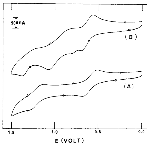
Figure 3. Cyclic voltammograms for (A) [\text{LMn}_2\text{Cl}_2]^{+1/2}\text{CH}_3\text{OH} (0.28 mM) and (B) [\text{LMn}_2\text{Br}_2]^{+1/2}\text{CH}_3\text{OH} (0.31 mM) dissolved in 1:1 \text{CH}_3\text{CN}/\text{CH}_2\text{Cl}_2 with 0.1 M [(n\text{-Bu})_4\text{N}]\text{ClO}_4 . The scan rate was 20 mV/s with a glassy carbon electrode. The potentials are referenced to a NHE. The IR drop has been compensated automatically by the instrument (BAS100).
