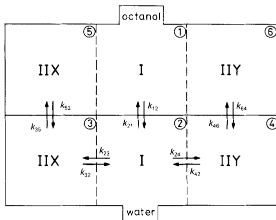
Fig. 1. Compartmental model describing the proxibarbal-valofan isomerisation and octanol/ H_2O partitioning. The numbers 1–6 refer to the six theoretical compartments in the model.
