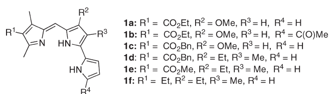
Figure 2. Pyrrolyldipyrins ( 1 ).
