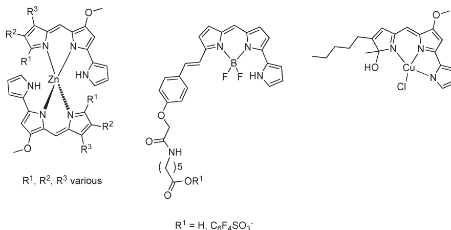
Figure 1. Complexes of pyrrolyldipyrins.
