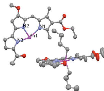
Figure 3. Thermal ellipsoid diagram (50%) of a twinned crystal of 2b. Sn(1) butyl groups and all hydrogen atoms are removed for clarity. Selected bond distances ( \text{\AA} ): Sn(1)–N(1), 2.309(2); Sn(1)–N(2), 2.128(2); Sn(1)–N(3), 2.239(2). Selected bond angles (deg): N(1)–Sn(1)–N(2), 81.46(9); N(1)–Sn(1)–N(3), 155.25(10); N(2)–Sn(1)–N(3), 73.85(10); C(43)–Sn(1)–C(47), 137.84(14) (C(43) and C(47) are the carbon atoms of each attached butyl group, respectively).
