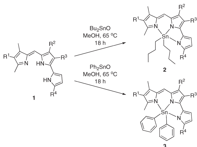
Scheme 1. General Synthetic Scheme for the Synthesis of Pyrrolyldipyrinato Sn(IV) Complexes
