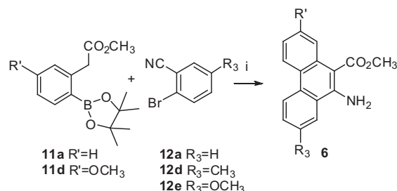
Scheme 4. Reverse general synthesis of 9-aminophenanthrenes. Reagents and conditions: (i) \text{Pd}(\text{PPh}_3)_4 cat 5%, \text{Cs}_2\text{CO}_3 3 equiv, DMF, 150^{\circ}\text{C} , MW.
