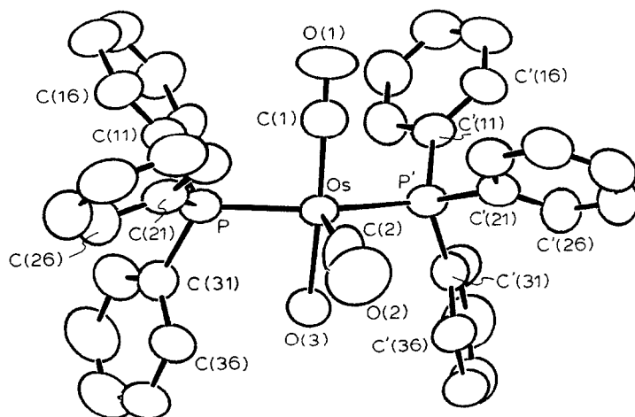
Fig. 1. Molecular structure of the cation in [\text{OsH}(\text{H}_2\text{O})(\text{CO})_2(\text{PPh}_3)_2][\text{BF}_4] \cdot \text{EtOH} , showing the crystallographic numbering. Primed atoms are generated by the symmetry operation x, \frac{1}{2} - y, z .
