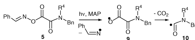
Scheme 4 Photodissociation of oxime oxalate amides.
