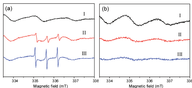
Figure 5. ESR spectra of (a) an N@C 60 /CuTPP mixture (molar ratio 1:1) and (b) a dyad 2N sample at (I) 4.1 \times 10^{-3} M, (II) 1.6 \times 10^{-3} M, and (III) 8.0 \times 10^{-4} M. Measurements were taken at room temperature in CS 2 , and the parameters were set to best demonstrate the signal of N@C 60 .
