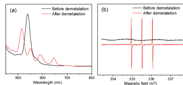
Figure 4. (a) UV-vis absorption and (b) ESR spectra of a dyad 2N sample before and after demetalation. The UV-vis spectra were recorded in a \text{CH}_2\text{Cl}_2 solution, and ESR spectra were recorded in a \text{CS}_2 solution.
