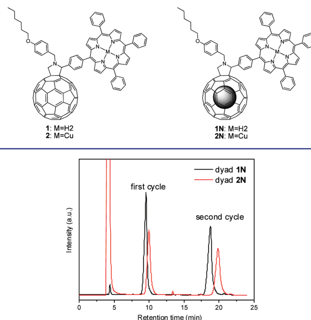
Figure 1. HPLC traces of dyads 1N (black) and 2N (red) (SPBB column, toluene as eluent, 18 mL/min).
