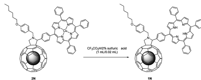
Scheme 1. Demetalation of Dyad 2N
