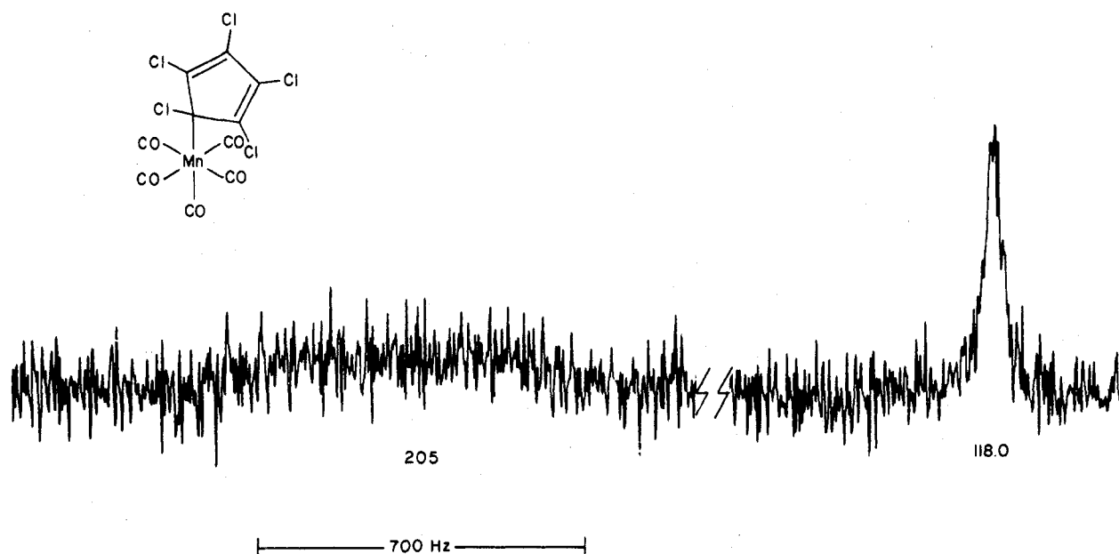
Figure 2. ^{13}\text{C} NMR spectrum of \text{Mn}(\eta^1\text{-C}_5\text{Cl}_5)(\text{CO})_5 in \text{CD}_2\text{Cl}_2 solution at 30^\circ\text{C} .
