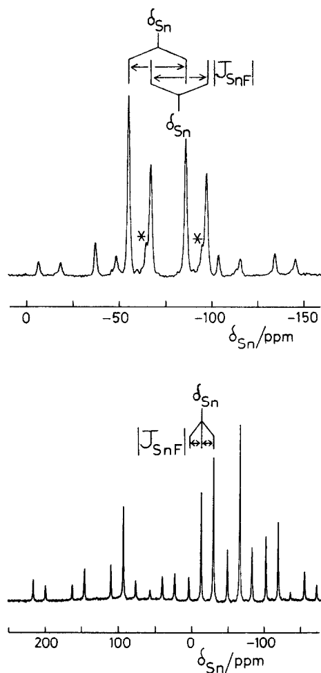
Fig. 3. Tin-119 CP-MAS spectra at 74.6 MHz of (below) t\text{-Bu}_3\text{SnF} (II) and (above) \text{Me}_3\text{SnF} (IV) to show the interpretation of the centrebands discussed in the text. The asterisks indicate the weak unassigned shoulders (see text). Spectrometer operating conditions: Contact time 5 ms; Recycle delay 2 s (II) and 5 s (IV); Number of transients 4134 (II) and 8626 (IV); Spinning speed 3090 Hz.
