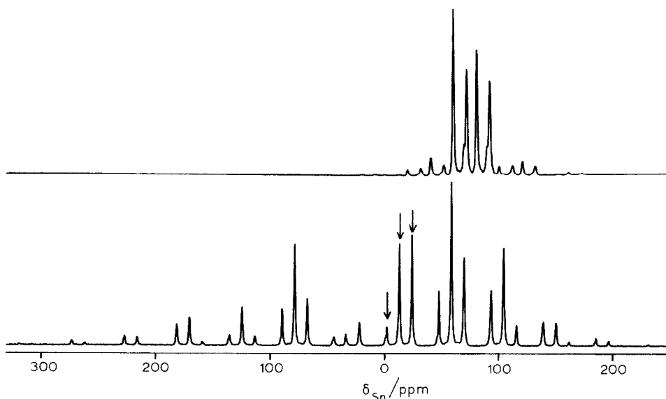
Fig. 1. Tin-119 CP-MAS NMR spectra at 111.9 MHz of (below) i\text{Bu}_3\text{SnF} (II) and (above) \text{Mes}_3\text{SnF} (IV), on the same scale. The centrebands for II are indicated by vertical arrows. Spectrometer operating conditions: Contact time 5 ms (II) and 2 ms (IV); Recycle delay 1 ms; Number of transients 2000 (II) and 5800 (IV); Spinning speed 5130 Hz (II) and 4420 Hz (IV).
