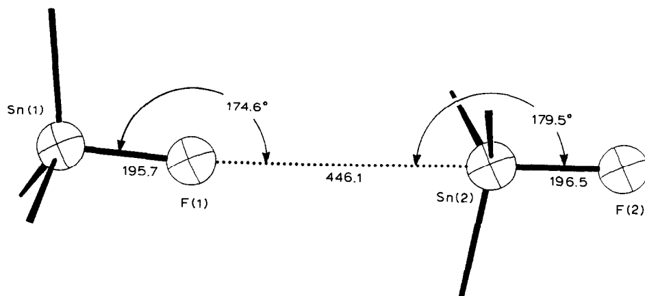
Fig. 2. Geometry of the crystallographic asymmetric unit for \text{Mes}_3\text{SnF} (IV) [8].
