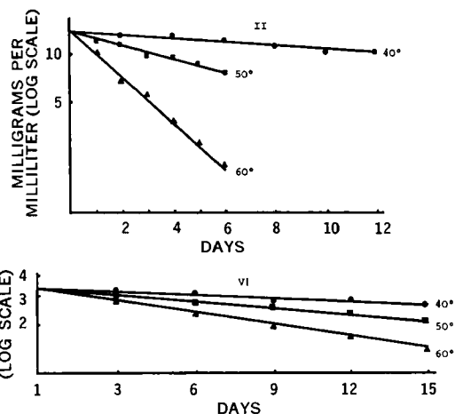
Figure 1 —Content of II or VI in aqueous solution. Initial concentration was: II, 14 mg/ml; and VI, 3.3 mg/ml. All data are the mean values of three experiments under the same conditions.
