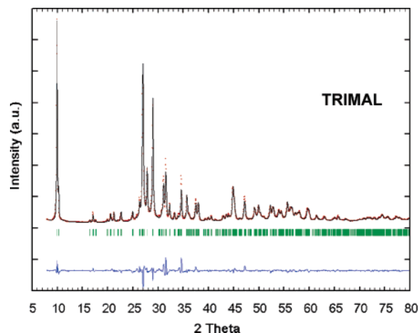
Figure 1. Observed (red dots), calculated (black line), and difference (blue line) Rietveld patterns for TRIMAL.
