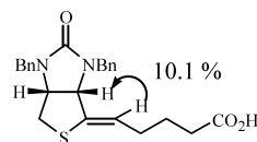
Fig. 1. ^1\text{H} -NMR Studies of NOE for Compound 8
