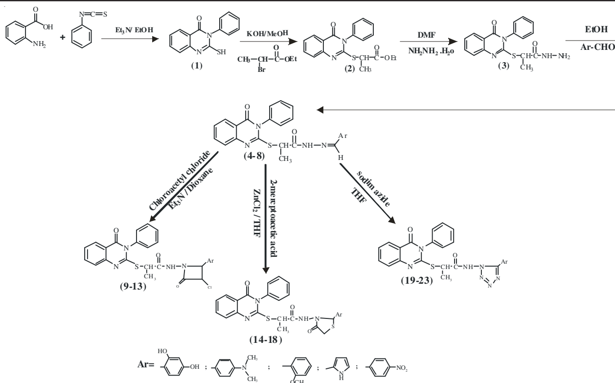
Scheme-I: Preparation of series of new 2-mercapto-3-phenyl-4(3H) quinazolinone, thiazolidine, azetidine and tetrazole
