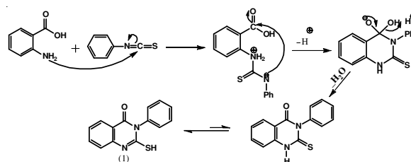
Mechanism of prepared compound 1
