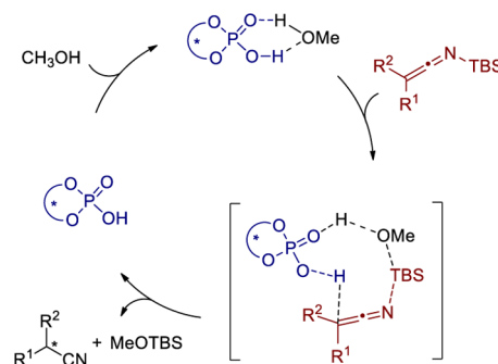
Scheme 2. Proposed Catalytic Cycle
