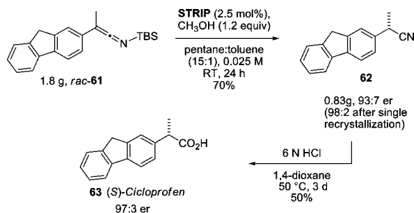
Scheme 1. Gram Scale Experiment and Enantioselective Synthesis of Cicloprofen
