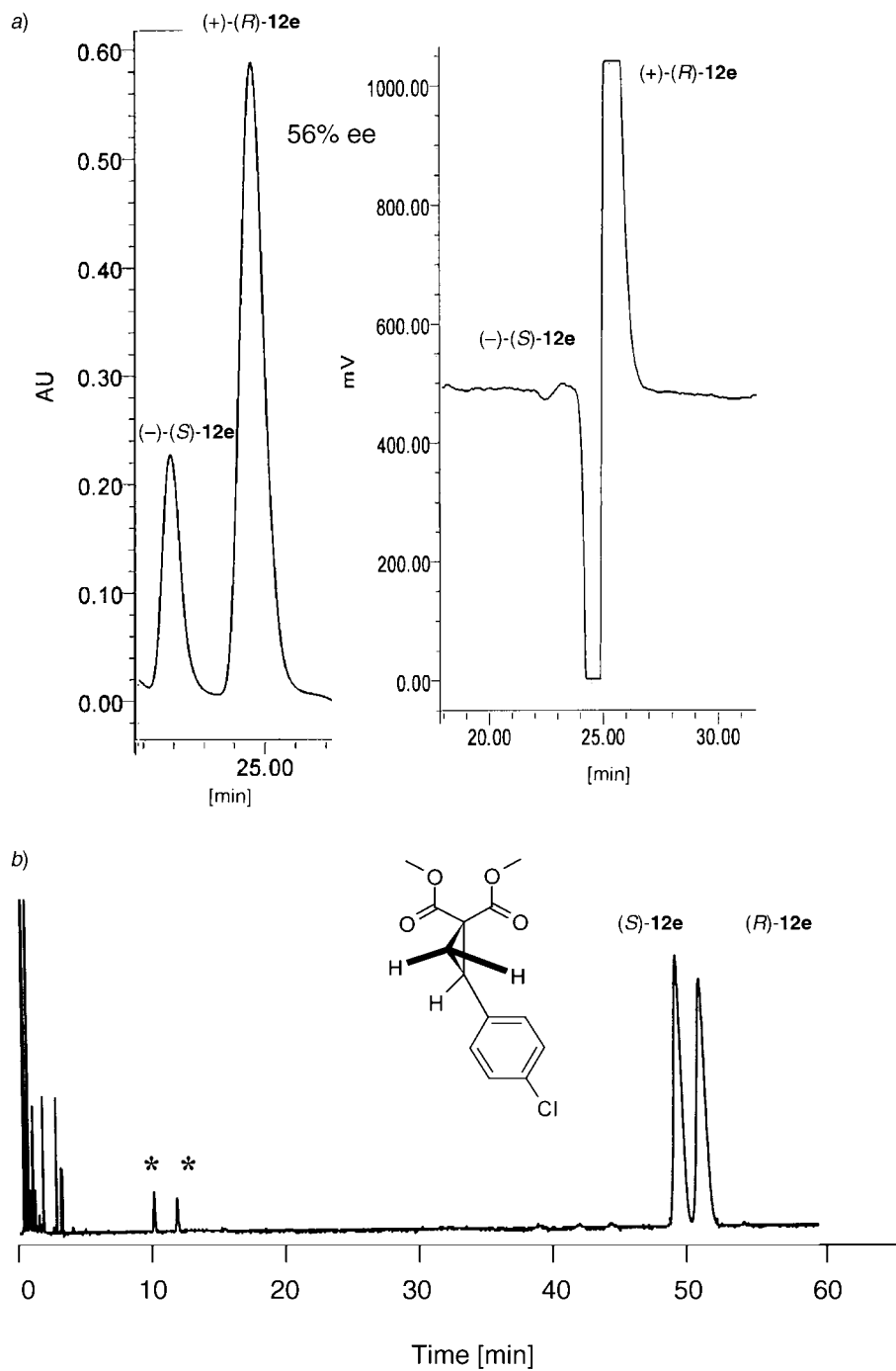
Fig. 7. Analysis of 12e : a) HPLC and b) GC. Cyclopropanation conditions: 5 + 3e , ylide precursor 7 , catalyst 10 . * = By-products (see Chapt. 2.3).
