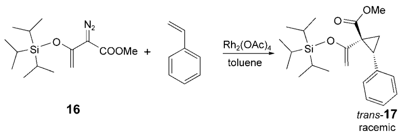
Scheme 3. Intermolecular Cyclopropanation of Styrene with 2-Diazo-3-(silyloxy)but-3-enoate 16
