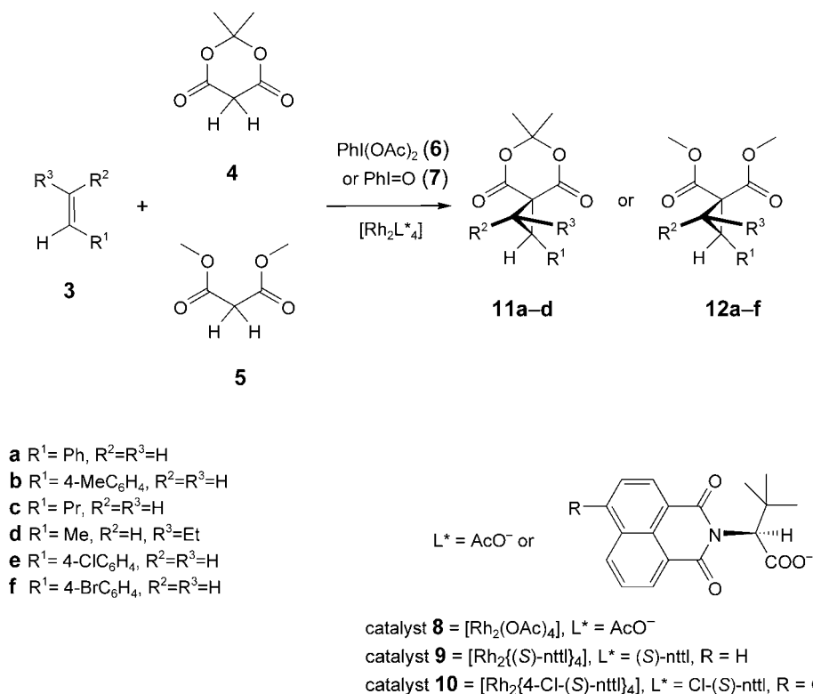
Scheme 1. One-Pot Synthesis of Cyclopropane Derivatives 11 and 12 from Meldrum's Acid ( 4 ) or Dimethyl Malonate ( 5 ), Respectively, and \text{PhI}(\text{OAc})_2 ( 6 ) or \text{PhI}=\text{O} ( 7 ), in Presence of the Achiral Rhodium(II) Catalyst 8 ( \text{L} = \text{AcO} ) or the Chiral Rhodium(II) Catalyst 9 ( \text{L} = (\text{S})\text{-nttl} ) or 10 ( \text{L} = 4\text{-Cl-(S)-nttl} )
