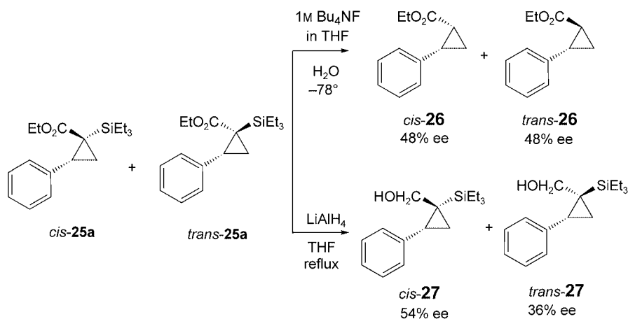
Scheme 6. Desilylation and Reduction of cis/trans -2-Phenyl-1-(triethylsilyl)cyclopropanecarboxylates cis/trans - 25a
