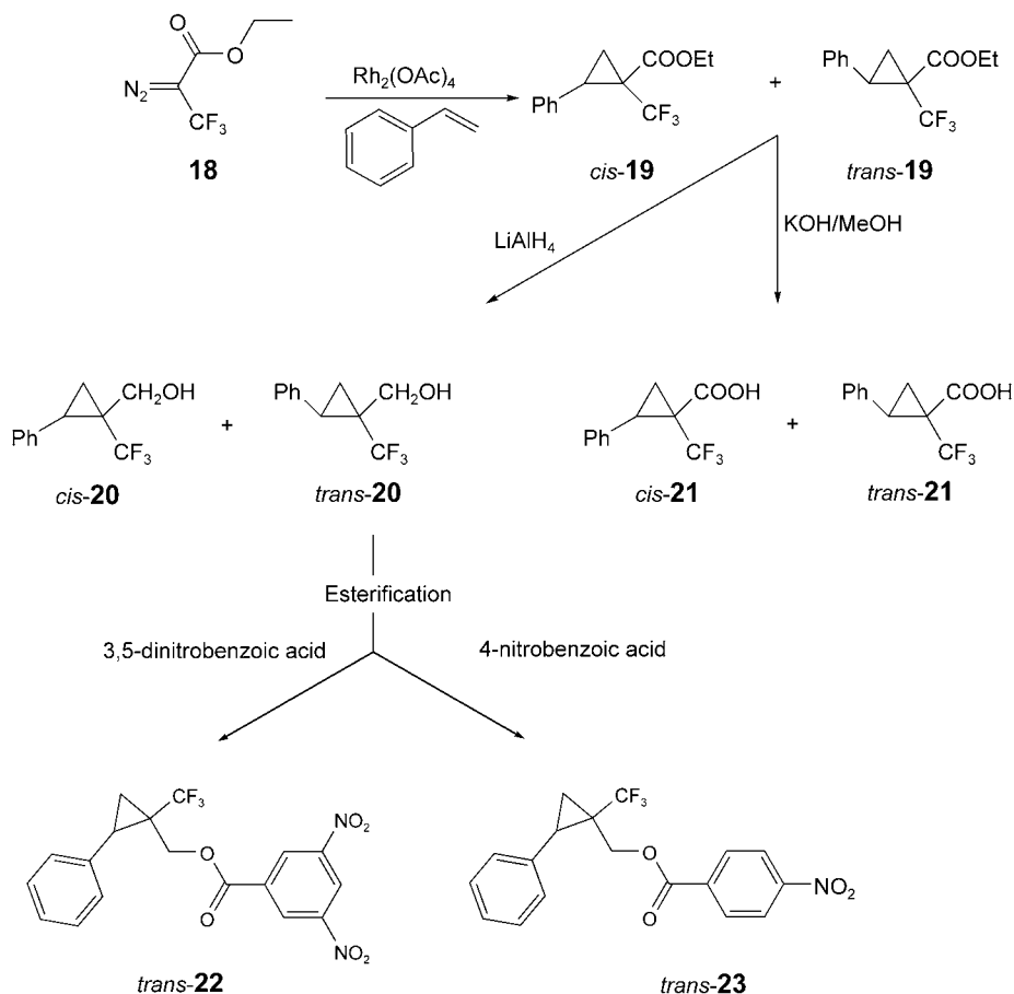
Scheme 4. Intermolecular Cyclopropanation of Styrene with 2-Diazo-3,3,3-trifluoropropanoate 18
