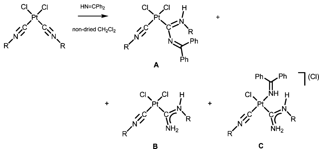
Scheme 2. Interplay between \text{Ph}_2\text{C}=\text{NH} and Pt-Bound Isonitrile Species Producing Aminoimino-Carbene and the Detected Decomposition and/or Side Products
