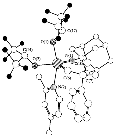
Figure 2. Chem 3D view of the structure of \text{Mo}(\text{NAd})(\text{CHCMe}_2\text{Ph})[\text{OCH}(\text{CF}_3)_2]_2(2,4\text{-lutidine}) ( 2a ).
