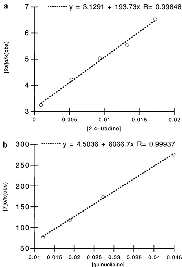
Figure 4. (a) Plot of [2a]_0/k_{\text{obs}} versus [2,4-lutidine] for polymerization of o -TMSPA; determination of k_{2a} and K_{2a} . (b) Plot of [7]_0/k_{\text{obs}} versus [quinuclidine] for polymerization of o -TMSPA; determination of k_7 and K_7 .
