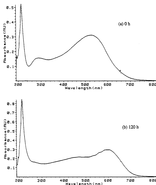
Figure 5. UV-vis spectra of (\text{o-TMSPA})_{10} in THF in the absence of air.
