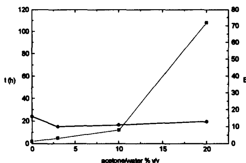
Fig. 2 Plot of acetone/water (%v/v) against the reaction time t(h) (■) and against the E (●) value at a reaction conversion of 30% at room temperature.
