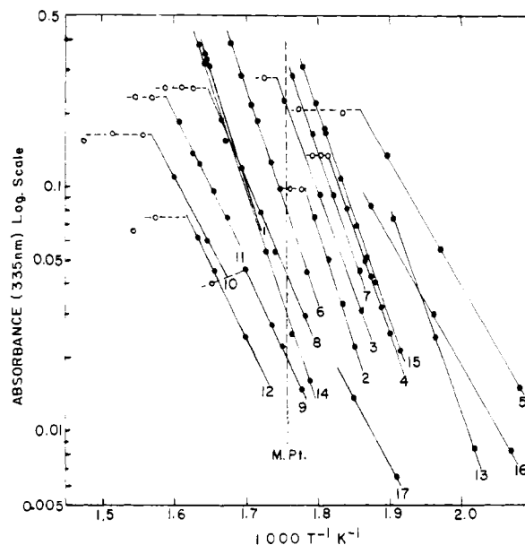
Figure 2. Temperature dependence of vapor-phase absorbances (as A_{\text{obsd}}/\text{path length} ) for various mixtures identified in Table I.
