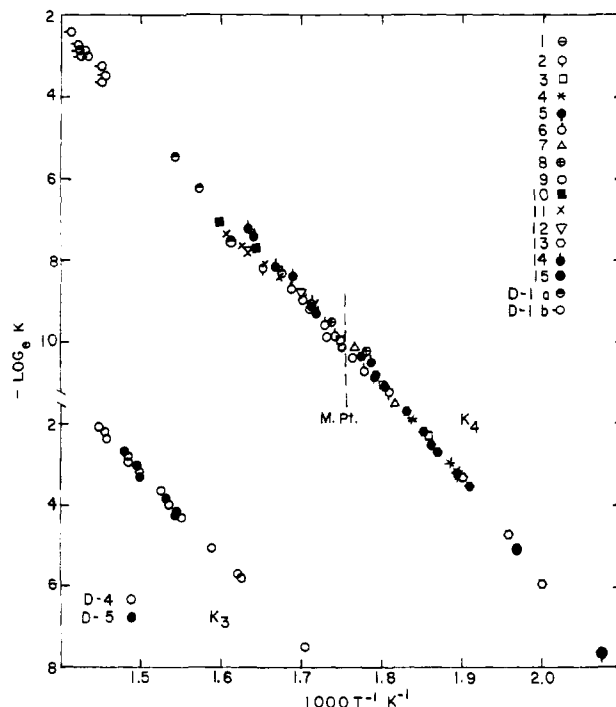
Figure 3. Temperature dependence of equilibrium constants for reactions 3 ( K_3 ) and 4 ( K_4 ) based on data from the various samples.
