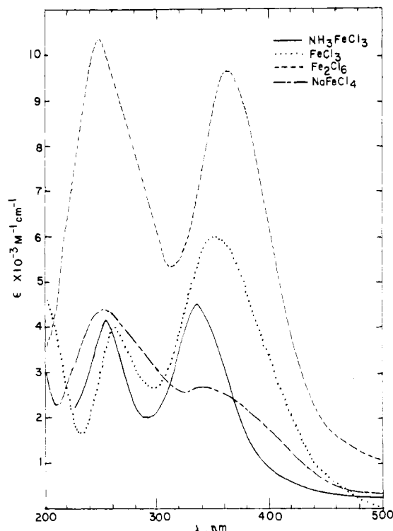
Figure 1. Tracing of the absorption spectrum of the vapor generated by \text{NH}_4\text{FeCl}_4 (attributed to \text{NH}_3\text{FeCl}_3 ) in comparison with \text{FeCl}_3(\text{g}) , \text{Fe}_2\text{Cl}_6(\text{g}) , and \text{NaFeCl}_4(\text{g}) .
