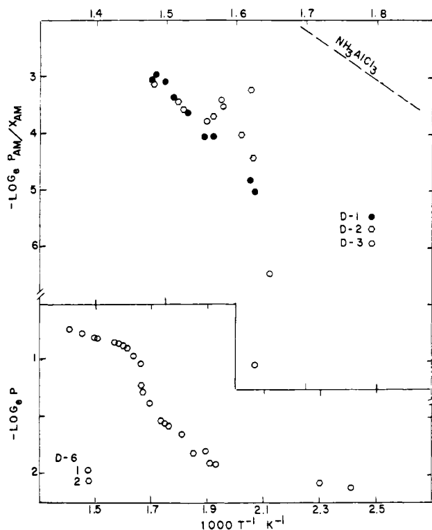
Figure 4. Top: Henry's law constants derived for \text{NH}_3\text{FeCl}_3 in \text{NH}_4\text{FeCl}_3 - \text{NH}_3\text{FeCl}_3 solutions in comparison with vapor pressure reported for \text{NH}_3\text{AlCl}_3 . Bottom: Variation of ammonia pressure with temperature in sample D-6 (pressure in atm).
