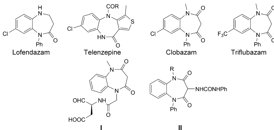
Figure. Important biologically active 1 H -1,5-benzodiazepines
