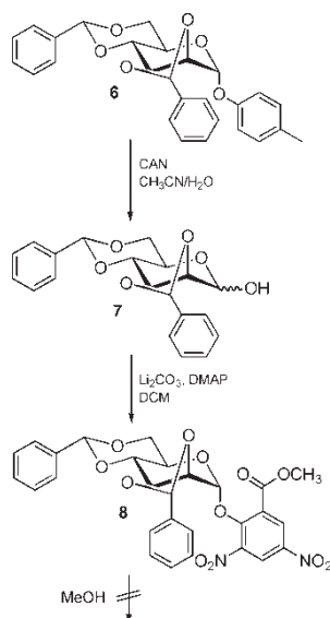
Scheme 3: Synthesis of 2,3:4,6-di- O -benzylidene-protected mannosyl DISAL derivative.
