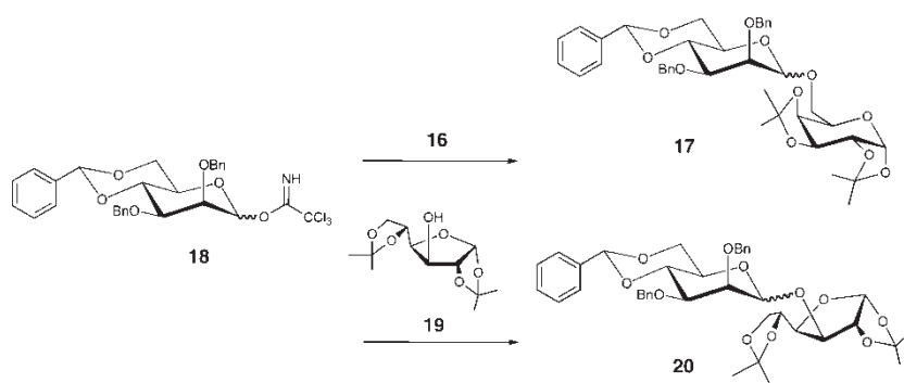
Scheme 6: O-Glycosylations with trichloroacetimidate donor 18 .
