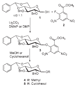
Scheme 2: Synthesis of benzylidene glucosyl DISAL donor 3 and its use in O -glycosylations.
