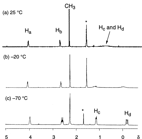
Fig. 2. Temperature dependent 1 H-NMR spectra of 1 (in CD 2 Cl 2 ; \pi -allyl ligand hydrogen region). Peaks with asterisks are due to impurities (probably water) contaminated during the sample preparation.
