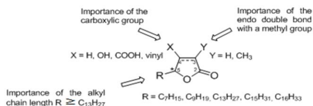
Figure 5. Pharmacomodulation
