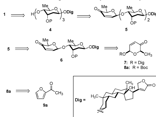
Scheme 1. Digitoxin Retrosynthetic Analysis
