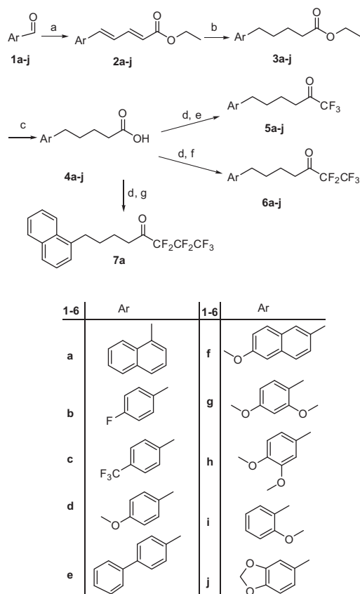
Scheme 1. Reagents and conditions: (a) C 2 H 5 OOCCH=CHCH 2 P(=O)(OC 2 H 5 ) 2 , LiOH, THF, reflux; (b) H 2 , 10% Pd/C, EtOH; (c) NaOH 1 N, EtOH; (d) (COCl) 2 , DMF, CH 2 Cl 2 ; (e) pyridine, (CF 3 CO) 2 O, CH 2 Cl 2 , 0 °C to rt; (f) pyridine, (CF 3 CF 2 CO) 2 O, CH 2 Cl 2 , 0 °C to rt; (g) pyridine, (CF 3 CF 2 CF 2 CO) 2 O, CH 2 Cl 2 , 0 °C to rt.
