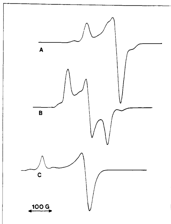
Figure 2. X-Band EPR spectra of tungsten(V)-oxo complexes (120 K, \sim 5 \times 10^{-4} M in DMF, 0.10 M (\text{C}_2\text{H}_5)_4\text{NCl} ): A, trans - \text{WOCl}_3(\text{bpy}) ; B, cis - \text{WOCl}(\text{ox})_2 ; C, cis - \text{WOCl}(\text{tox})_2 .
