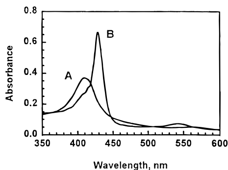
Figure 4. (A) Visible spectrum of mononitroiron(III) picket fence porphyrin, [Fe III TpivPP(NO 2 )] ( 1.5 \times 10^{-5} M), in acetonitrile, path length = 1 cm, sealed under nitrogen. (B) Change in visible spectrum A upon reaction with NO (7.5 mM), obtained by immediate collection of the spectrum after injection of an equal volume of saturated NO solution in acetonitrile and correcting for dilution.
