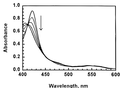
Figure 3. Visible spectra accompanying the decomposition of [\text{Fe}^{\text{II}}\text{TpivPP}(\text{NO})(\text{NO}_2)]^- ( 2 ), shown in Figure 1B, to [\text{Fe}^{\text{II}}\text{TpivPP}(\text{NO})] ( 8 ) under anaerobic conditions. Spectra acquired in the order indicated by the arrow were collected at times of 30 sec, 24 min, 57 min, 90 min, and 7 h.
