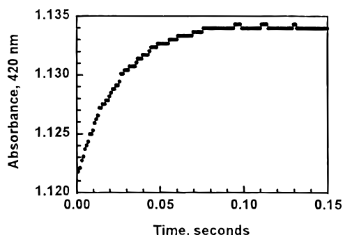
Figure 2. Rapid absorbance change accompanying the reaction of the dinitroiron(III) picket fence porphyrin anion, [\text{Fe}^{\text{III}}\text{TpivPP}(\text{NO}_2)_2]^- ( 1 ), with triphenylphosphine in acetonitrile/TPA/ClO 4 medium, obtained by stopped-flow spectrophotometry under nitrogen. Observation wavelength = 420 nm, porphyrin concentration = 7.5 \times 10^{-5} M, [(\text{TPA})\text{NO}_2] = 5 \times 10^{-3} M, [\text{Ph}_3\text{P}] = 2.5 \times 10^{-2} M; observation path length = 6.2 mm.
