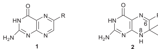
Scheme 1. Reagents: Pterin compounds: (a) R is absent, (b) R=CH 3 , (c) R=CH 2 OH, (d) R=OH, and (e) R=CH 2 NHR'.
