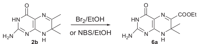
Scheme 4. Preparation of 6-carboxylic ethyl ester-7,7-dimethyl-7,8-dihydropterin ( 6a ).
