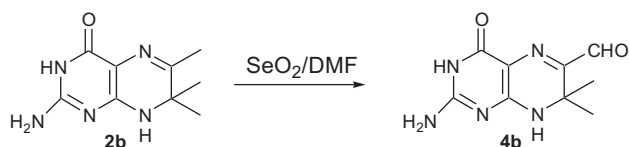
Scheme 3. New method of deriving 6-aldehyde-7,7-dimethyl-7,8-dihydropterin ( 4b ) from 6,7,7-trimethyl-7,8-dihydropterin ( 2b ).
