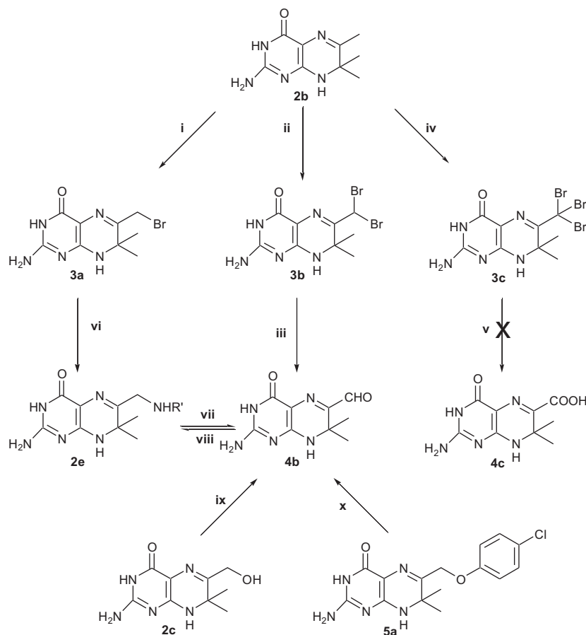
Scheme 2. Derivatization of compound 2b : (i, ii) as reported, 13,14 (iii–viii) this work, (ix, x) as reported. 23,12
