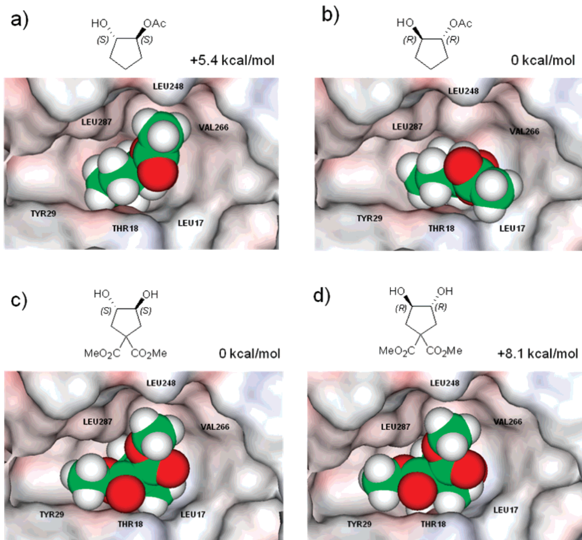
FIGURE 2. Computer modeling of transition state analogue–Amano PS complexes. (a, b) Modeling of the transition state analogue of plain ( S,S )- and ( R,R )-monoacetate in the active site of Amano PS. The ( R,R )-enantiomer was more stable than the ( S,S )-enantiomer by 5.4 kcal/mol. (c, d) Modeling of the transition state analogue of ( S,S )- and ( R,R )-diol 3 having a diester moiety in the active site. A hydrogen bond between the diester moiety and Thr18 is observed. The ( S,S )-enantiomer was more stable than the ( R,R )-enantiomer by 8.1 kcal/mol.
