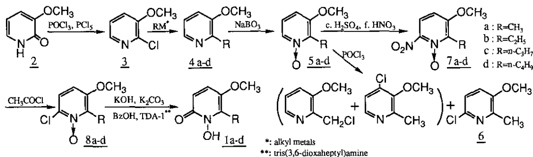
Scheme 1. Synthetic Route of 2-Alkyl-6-hydroxy-3-methoxypyridine 1-Oxides.
