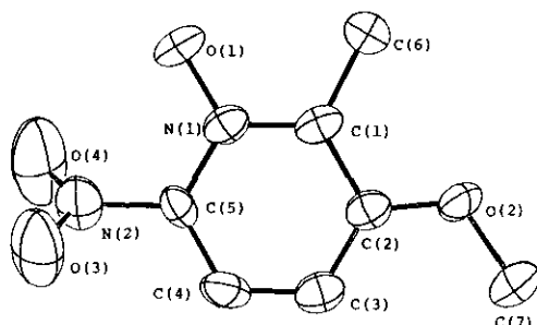
Fig. 1. X-Ray Diffraction of 3-Methoxy-2-methyl-6-nitropyridine 1-Oxide ( 7a ).
