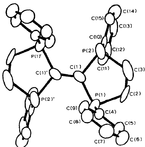
Fig. 1. The molecular structure of [(\text{PhPCH}_2\text{CH}_2\text{P(Ph)C=})_2] (I). Selected bond lengths: C(1)–C(1)', 1.352(15); P(1)–C(1), 1.846(10); P(1)–C(2), 1.844(14); P(1)–C(4), 1.806(13); P(2)–C(1), 1.834(13); P(2)–C(3), 1.848(12); P(2)–C(10), 1.854(14) Å. Selected bond angles: C(1)–P(1)–C(2), 94.7(6); C(1)–P(1)–C(4), 103.8(5); C(2)–P(1)–C(4), 99.3(6); C(1)–P(2)–C(3), 93.3(6); C(1)–P(2)–C(10), 105.1(6); C(3)–P(2)–C(10), 99.6(6); P(1)–C(1)–P(2), 114.8(6); P(1)–C(1)–C(1)', 122.4(9); P(2)–C(1)–C(1)', 122.8(8)°.
