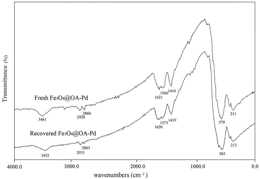
Fig. 3 FT-IR spectra of fresh and recovered \text{Fe}_3\text{O}_4@\text{OA-Pd}
