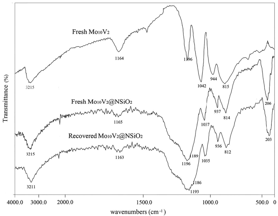
Fig. 4 FT-IR spectra of fresh and recovered \text{Mo}_{10}\text{V}_2@\text{NSiO}_2 and fresh \text{Mo}_{10}\text{V}_2
