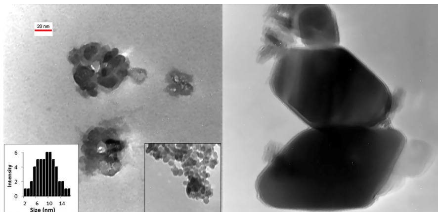
Fig. 1 TEM images and size distribution of Fe 3 O 4 @OA-Pd
