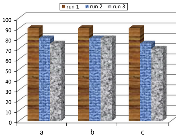
Fig. 5 Reusability of \text{Fe}_3\text{O}_4\text{@OA-Pd} and \text{Mo}_{10}\text{V}_2\text{@NSiO}_2 in the model reaction (after 8 h). a Model reaction with recovered \text{Mo}_{10}\text{V}_2\text{@NSiO}_2 . b Model reaction with recovered \text{Fe}_3\text{O}_4\text{@OA-Pd} . c Model reaction with recovered \text{Mo}_{10}\text{V}_2\text{@NSiO}_2 and \text{Fe}_3\text{O}_4\text{@OA-Pd}
