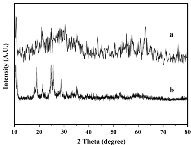
Fig. 2 XRD patterns of a Mo 10 V 2 @NSiO 2 and b PMo 10 V 2
