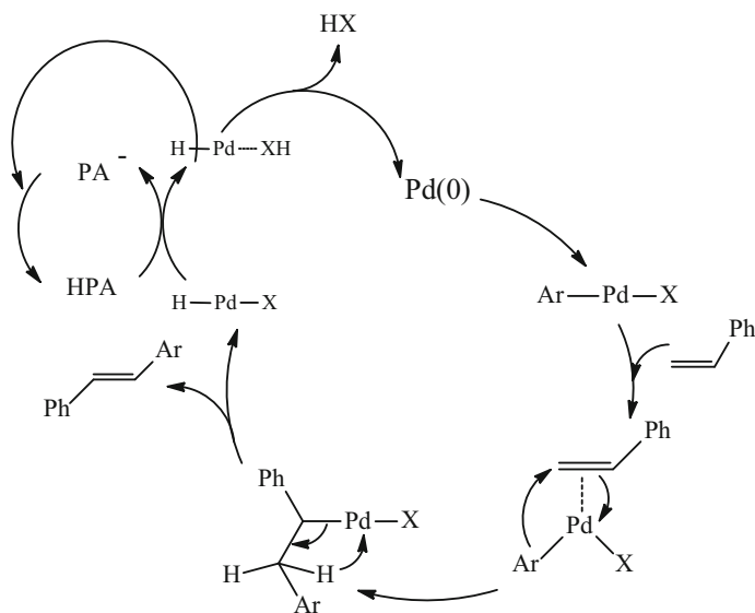
Scheme 2 Proposed mechanism for Heck reaction catalyzed by \text{Fe}_3\text{O}_4\text{@OA-Pd} and \text{Mo}_{10}\text{V}_2\text{@NSiO}_2
