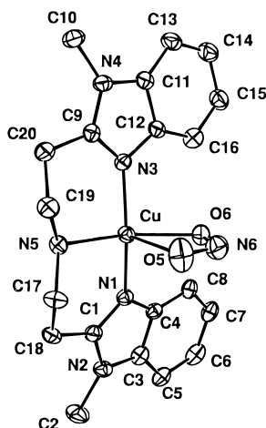
Figure 5. View of the [\text{Cu}(2\text{-BB})(\text{NO}_2)]^+ cation in the [\text{Cu}(2\text{-BB})(\text{NO}_2)](\text{ClO}_4)(\text{MeCN}) crystal.
