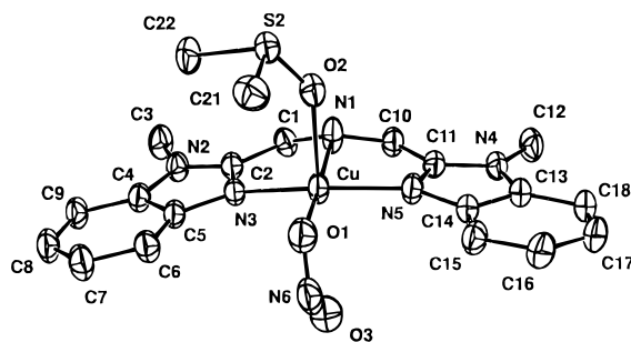
Figure 2. View of the [\text{Cu}(\text{1-BB})(\text{DMSO-O})(\text{NO}_2)]^+ cation in the [\text{Cu}(\text{1-BB})(\text{DMSO-O})(\text{NO}_2)](\text{ClO}_4) crystal.
