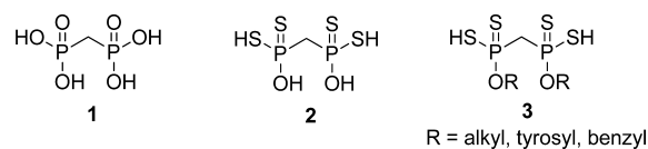
Figure 1. Structures of MDP 1 , MDTP 2 , and O,O'-diester-methylenediphosphonetetrathioate derivatives 3 .
