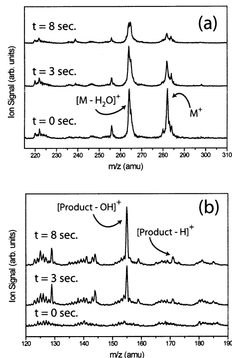
Figure 3. Mass spectra digitized at high resolution for particles of radius 2.45\ \mu\text{m} with P_{\text{O}_3} = 1.3 \times 10^{-4}\ \text{atm} and reaction times of 0, 3, and 8 s: (a) high-mass peaks including molecular ion of oleic acid ( \text{M}^+ ) at m/z = 282 , (b) low-mass peaks showing emergence of peaks at m/z = 171 and m/z = 155 .
