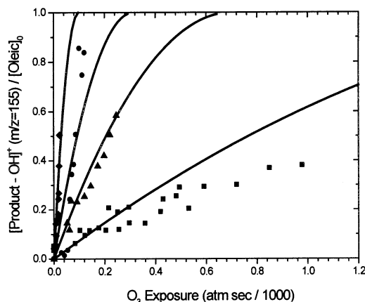
Figure 8. Rise of peak at m/z = 155 as a function of \text{O}_3 exposure ( P_{\text{O}_3}t ) for four particle sizes: \diamond 680 nm, \bullet 1.38 \mu\text{m} , \blacktriangle 1.86 \mu\text{m} , \blacksquare 2.45 \mu\text{m} . Lines represent expected signal if every oleic acid molecule that reacts results in the creation of a fragment at m/z = 155 .
