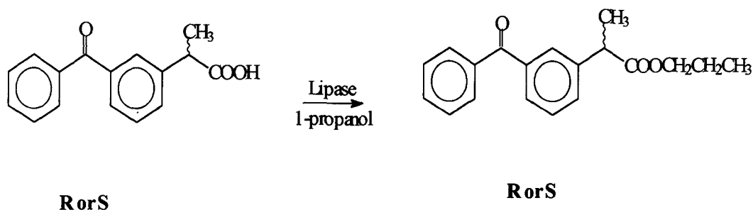
Scheme 2.- Enantioselective esterification of (R) or (S) Ketoprofen.
