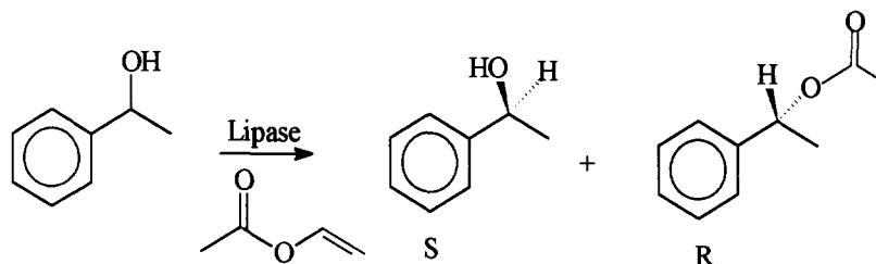
Scheme 3.- Enzymatic transesterification of ( R,S )-1-phenyl-ethanol.
