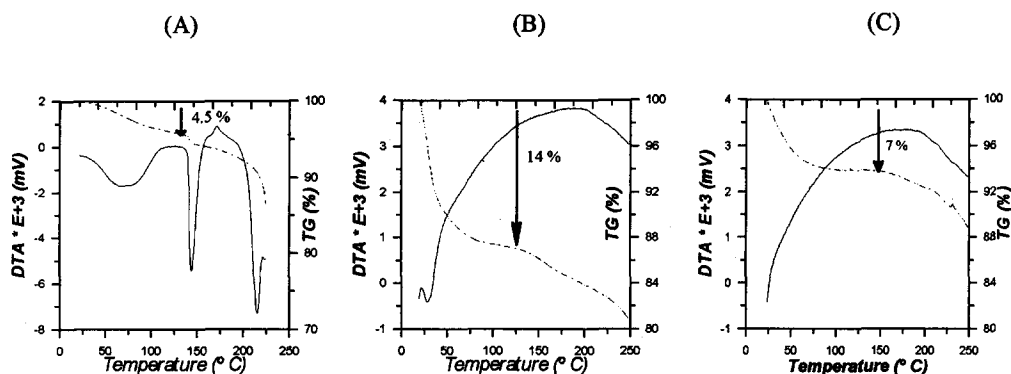
Figure 1.- Curves of TGA (---) and DTA (—) of several lipases: A) Commercial lipase (L85), and pure isoenzymes, B) Lipase A and C) Lipase B.
