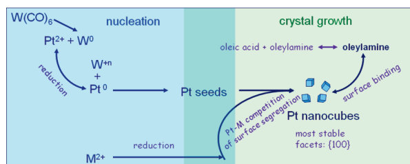
Scheme 1. Illustration of Both Nucleation and Crystal Growth Processes for \text{Pt}_3\text{M} Nanocubes (M = Co, Fe, and Ni)
