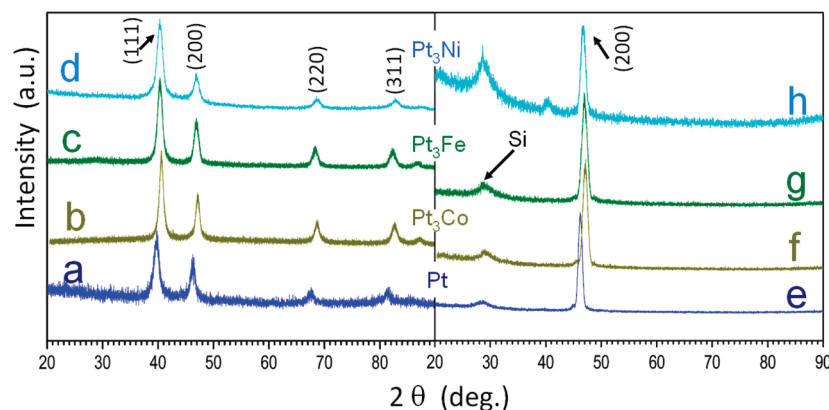
Figure 3. XRD pattern of \text{Pt}_3\text{M} nanocubes: (a,e) Pt, (b,f) \text{Pt}_3\text{Co} , (c,g) \text{Pt}_3\text{Fe} , and (d,h) \text{Pt}_3\text{Ni} . (a–d) Samples were randomly deposited on a PANalytical zero-background Si sample holder. (e–h) Samples were assembled on a surface-polished 25 mm Si (100) wafer.
