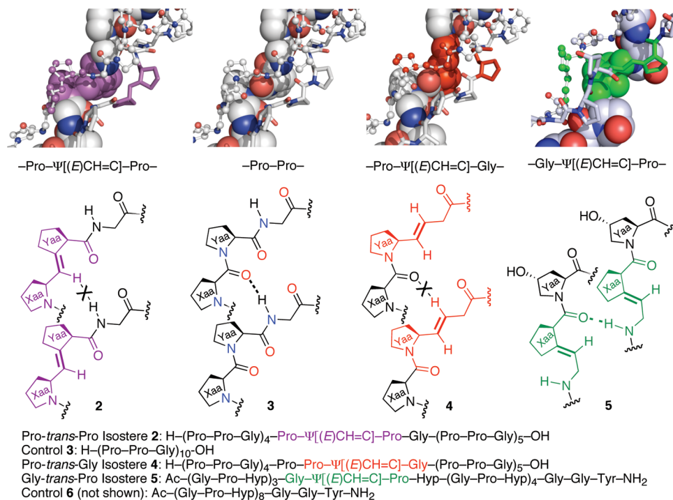
Figure 1. Pro- trans -Pro ( E )-alkene isostere containing collagen host–guest peptide 2, control 3, Pro- trans -Gly isostere peptide 4, 22 Gly- trans -Pro isostere peptide 5, and its control 6 (not shown). 23 The ( E )-alkene isosteres and interchain hydrogen-bonding patterns (---), or lack thereof (X), are shown in the structures.
