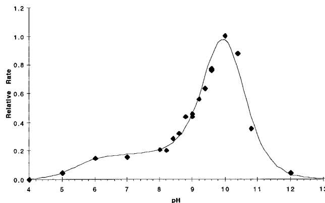
Figure 3. pH-rate dependence of oleamide hydrolase cleavage of 1 , with the fit showing apparent active site \text{pK}_a values of 5.4, 9.7, and 10.3. The rate maximum occurs at pH 10.0.
